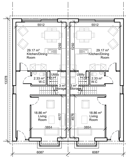
1 Ground Floor Plan 0400
